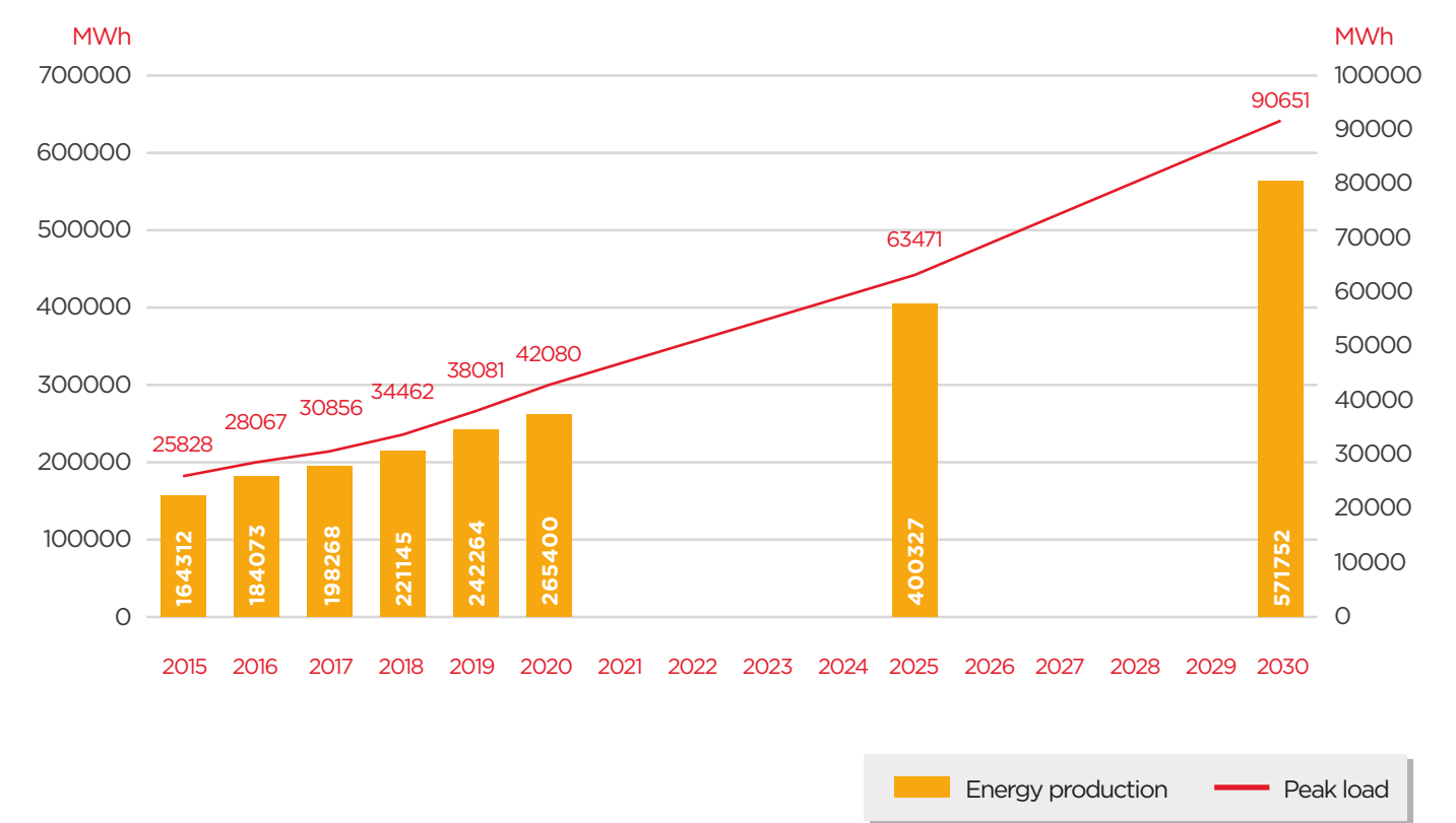
Energy Production (MWh) and Peak load (MW) from 2015 to 2030
